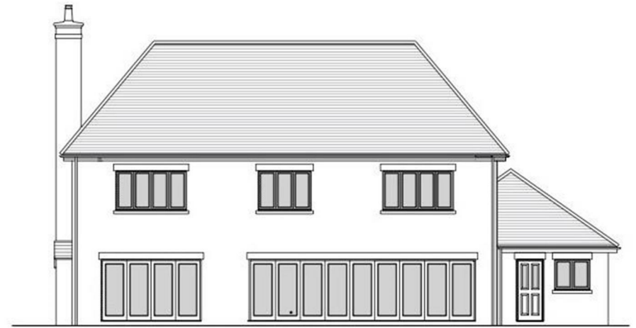
SOUTH ELEVATION AS PROPOSED
